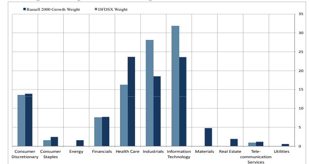
Portfolio Weights - DFDSX Weight vs. Russell 2000 Growth Weight
